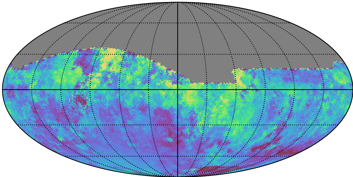
too_5_1v3.4_10yrs All sky i band: Median moonDistance
