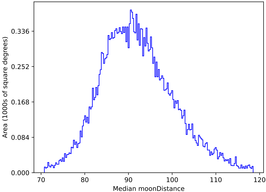
too_5_1v3.4_10yrs All sky i band: Median moonDistance
