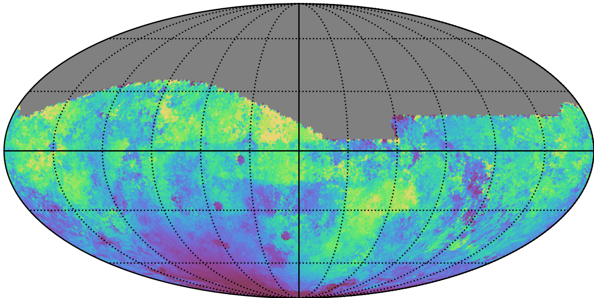
too_5_1v3.4_10yrs All sky g band: Median moonDistance
