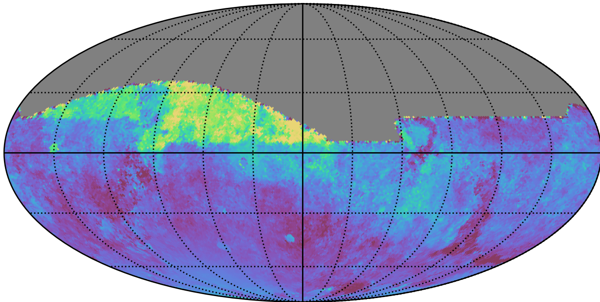
too_5_1v3.4_10yrs All sky all bands: Median moonDistance
