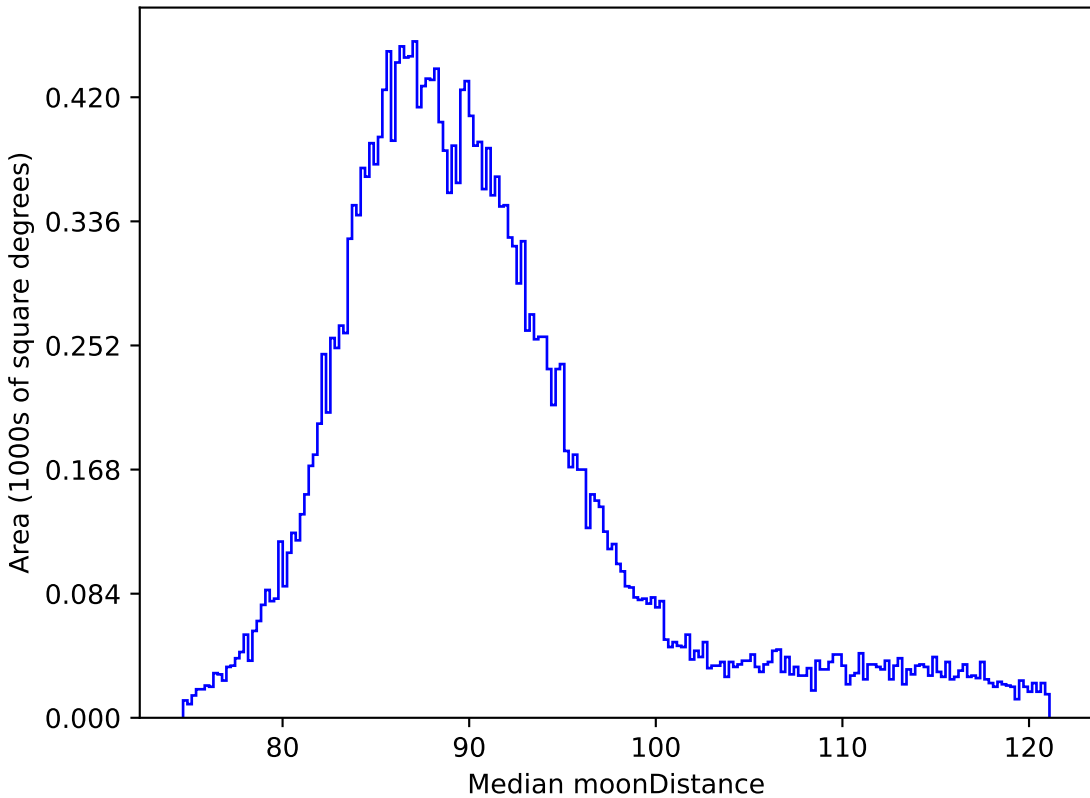
too_5_1v3.4_10yrs All sky all bands: Median moonDistance
