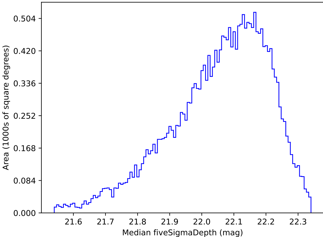
too_5_1v3.4_10yrs Yr 1 y band: Median fiveSigmaDepth
