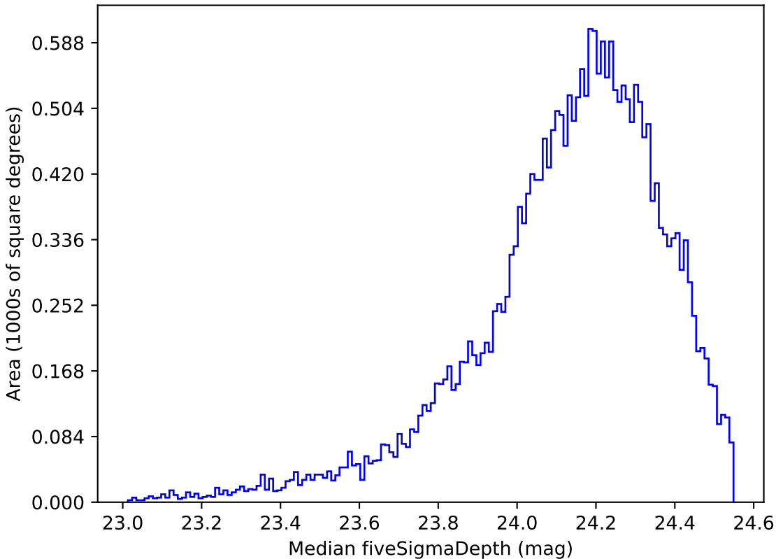
too_5_1v3.4_10yrs Yr 1 r band: Median fiveSigmaDepth
