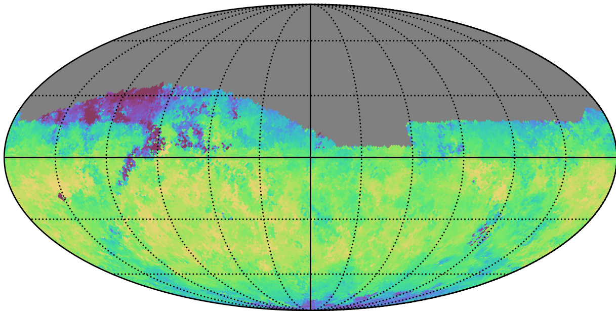
too_5_1v3.4_10yrs Yr 1 i band: Median fiveSigmaDepth
