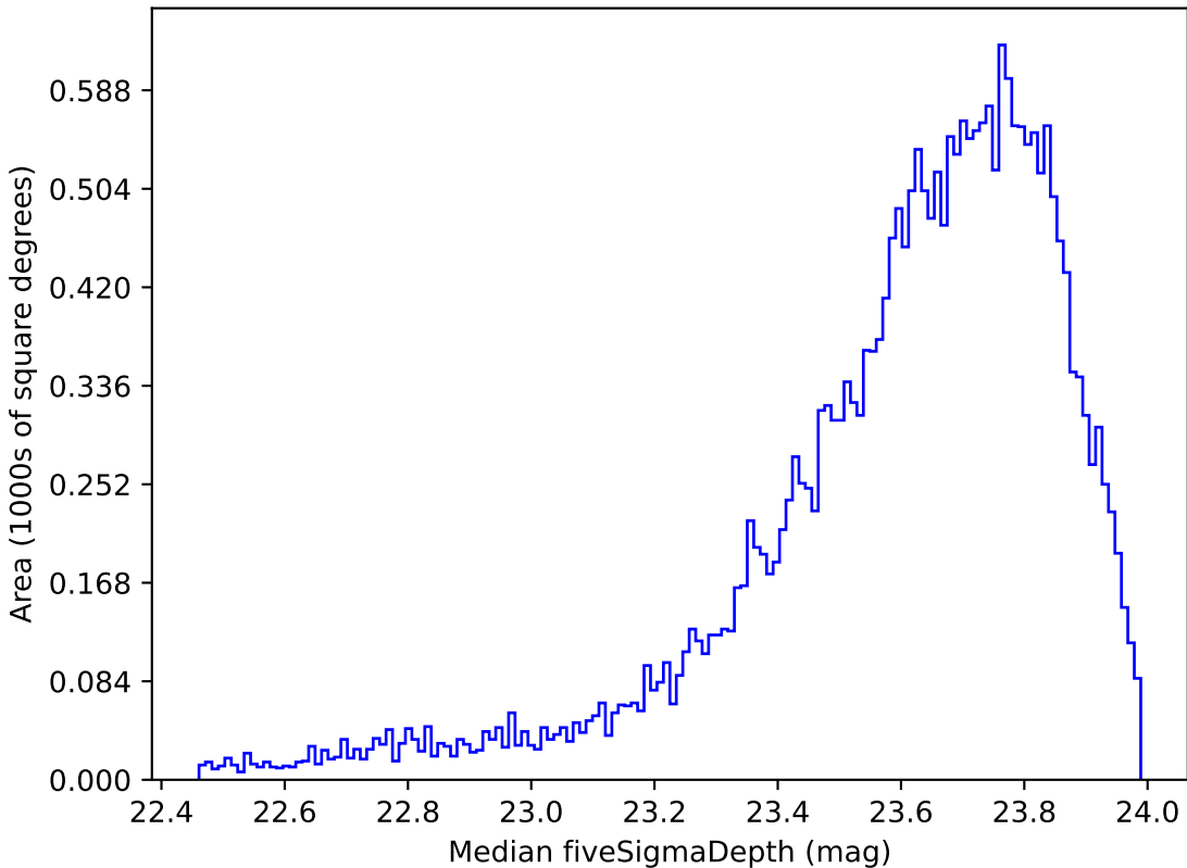
too_5_1v3.4_10yrs Yr 1 i band: Median fiveSigmaDepth
