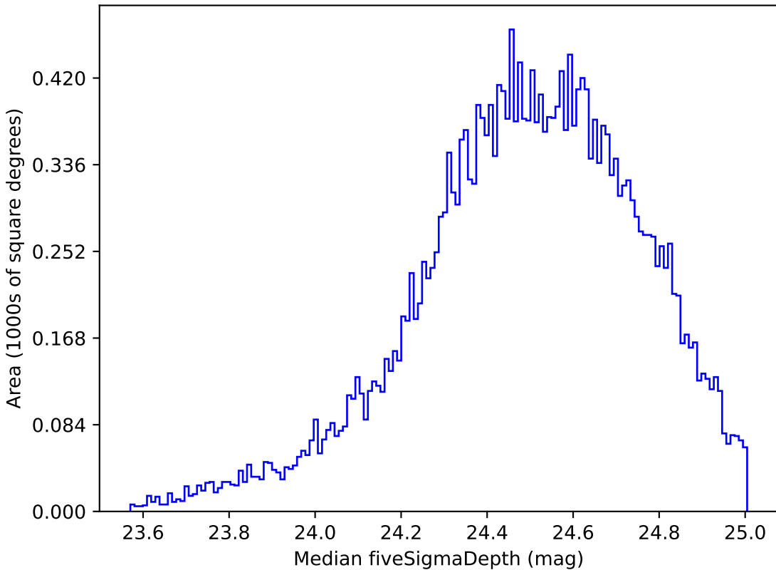
too_5_1v3.4_10yrs Yr 1 g band: Median fiveSigmaDepth
