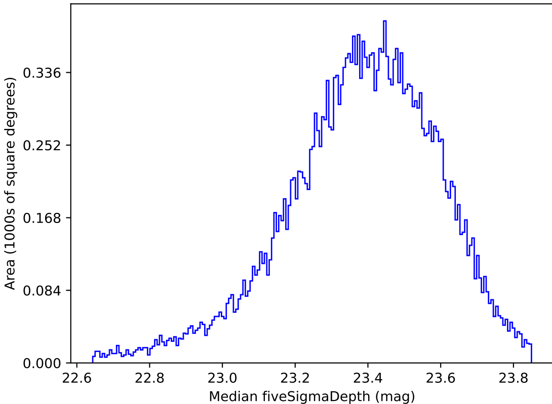
too_5_1v3.4_10yrs Yr 1 all bands: Median fiveSigmaDepth
