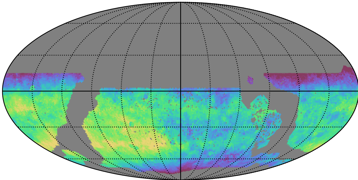
too_5_1v3.4_10yrs WFD z band: Median fiveSigmaDepth
