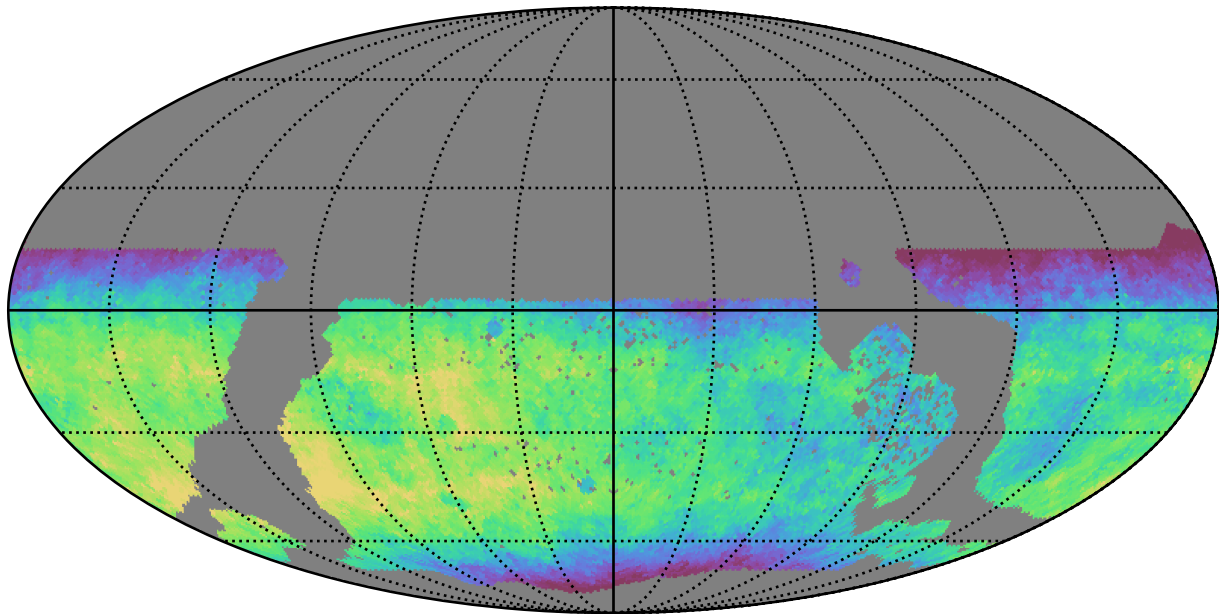
too_5_1v3.4_10yrs WFD y band: Median fiveSigmaDepth
