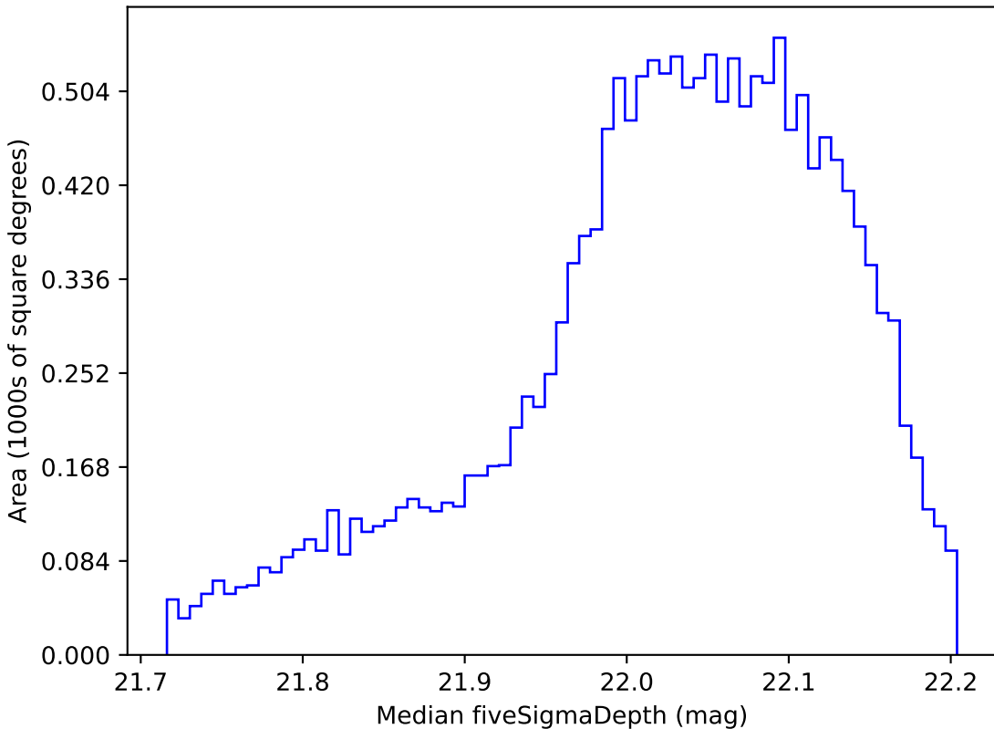
too_5_1v3.4_10yrs WFD y band: Median fiveSigmaDepth
