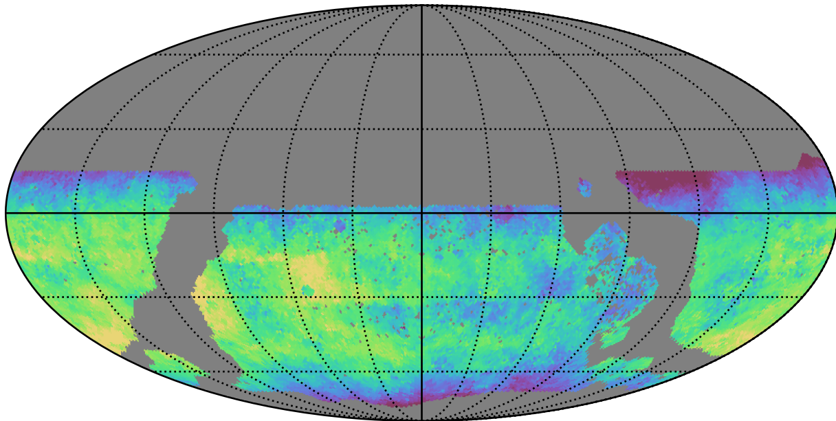
too_5_1v3.4_10yrs WFD u band: Median fiveSigmaDepth
