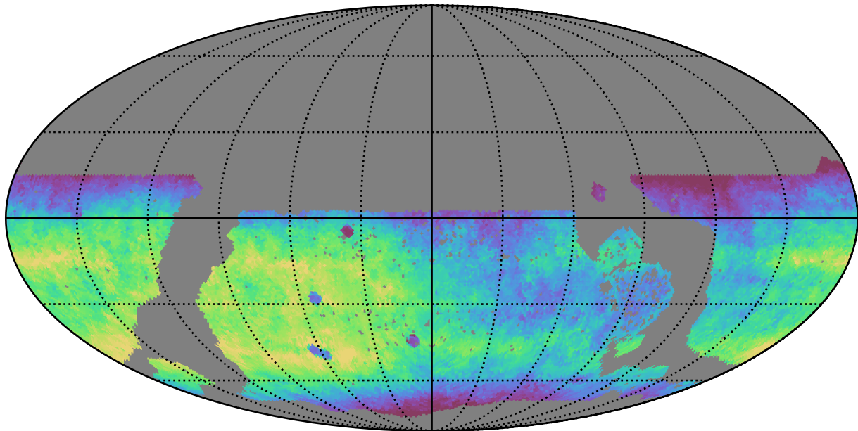
too_5_1v3.4_10yrs WFD r band: Median fiveSigmaDepth
