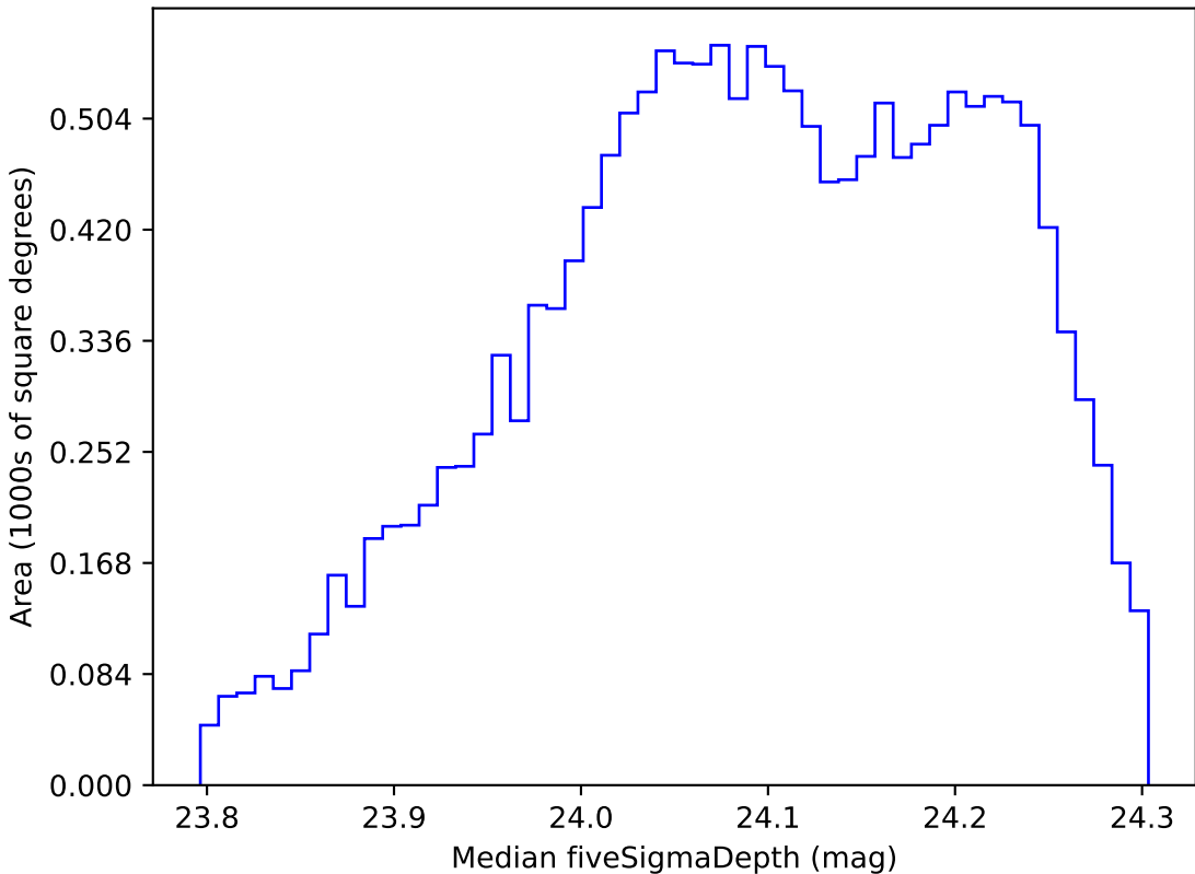
too_5_1v3.4_10yrs WFD r band: Median fiveSigmaDepth
