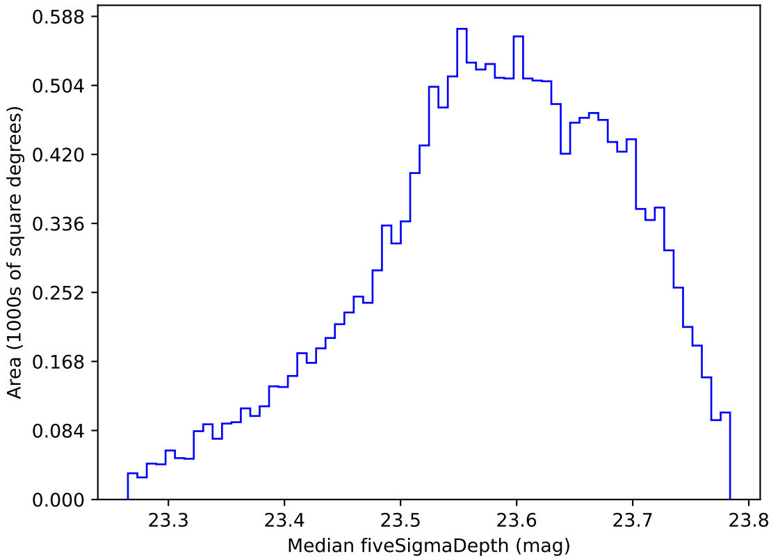
too_5_1v3.4_10yrs WFD i band: Median fiveSigmaDepth
