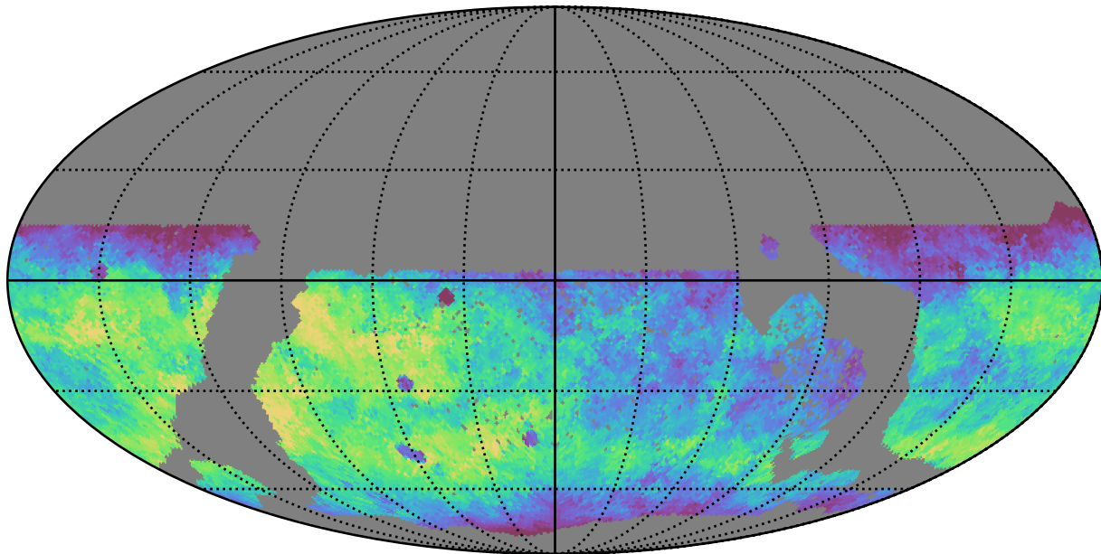
too_5_1v3.4_10yrs WFD g band: Median fiveSigmaDepth
