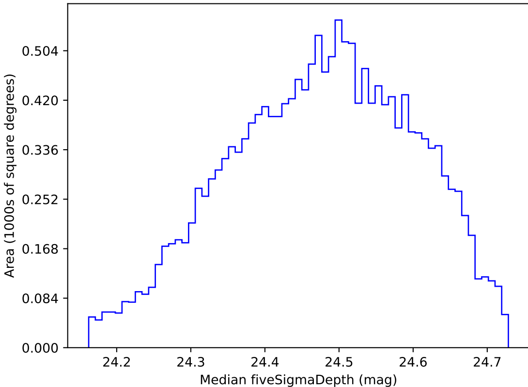
too_5_1v3.4_10yrs WFD g band: Median fiveSigmaDepth
