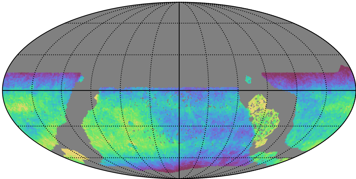
too_5_1v3.4_10yrs WFD all bands: Median fiveSigmaDepth
