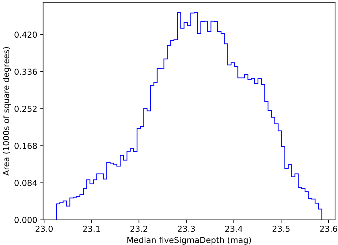
too_5_1v3.4_10yrs WFD all bands: Median fiveSigmaDepth
