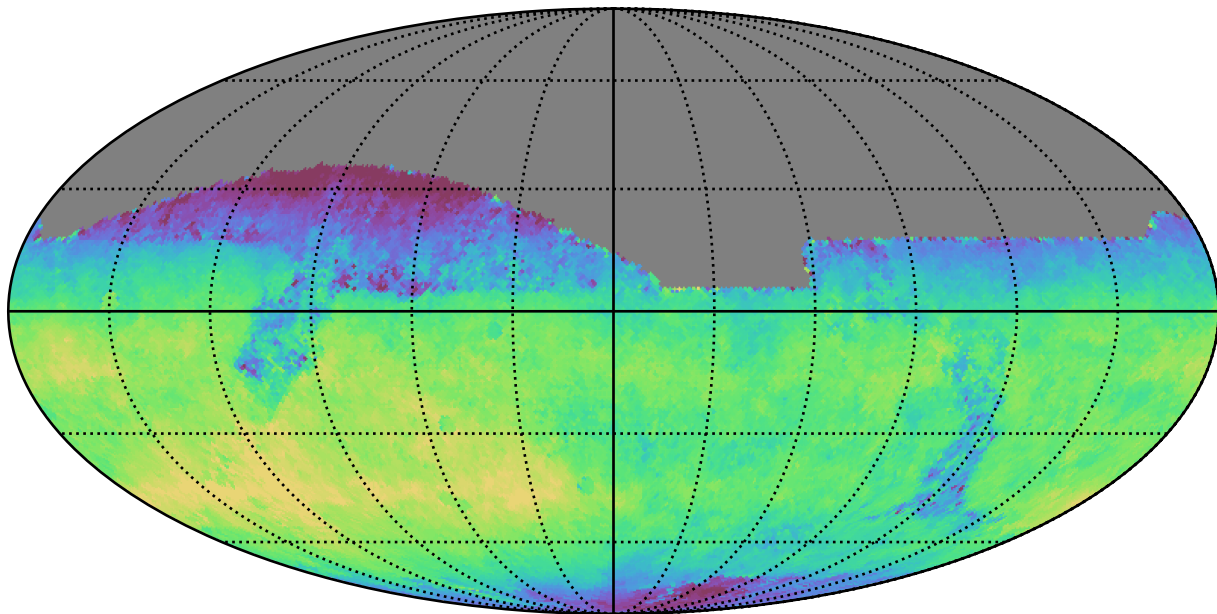
too_5_1v3.4_10yrs All sky z band: Median fiveSigmaDepth
