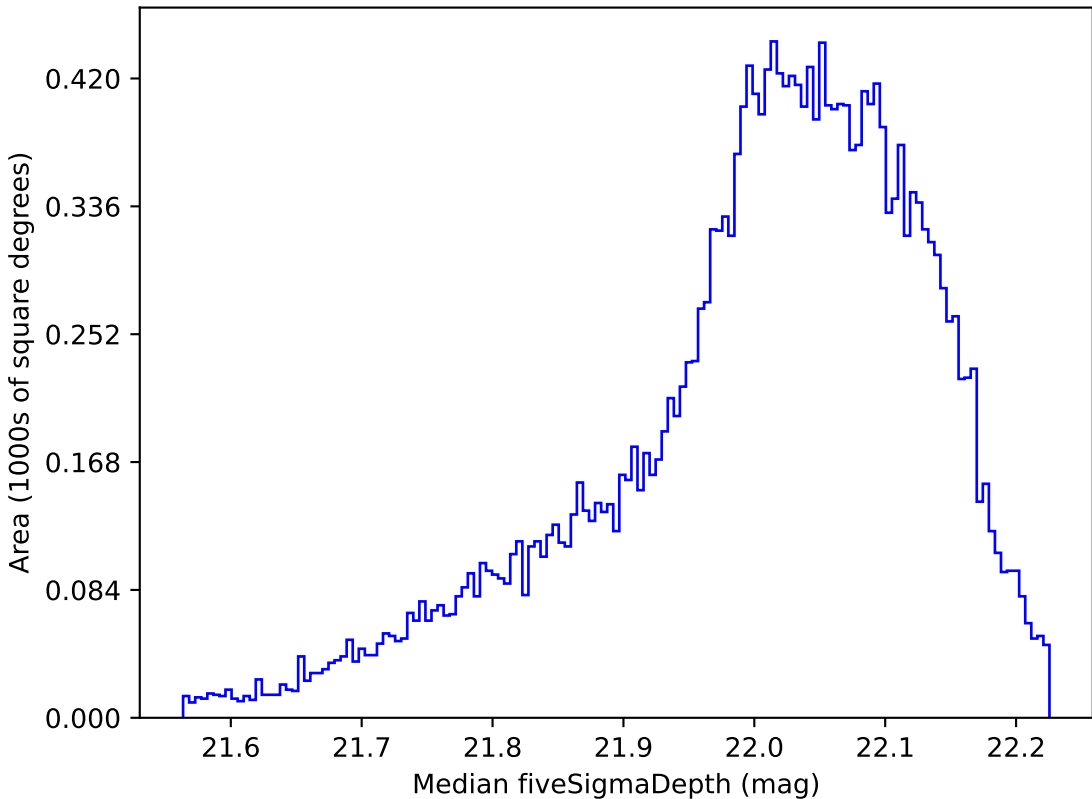
too_5_1v3.4_10yrs All sky y band: Median fiveSigmaDepth
