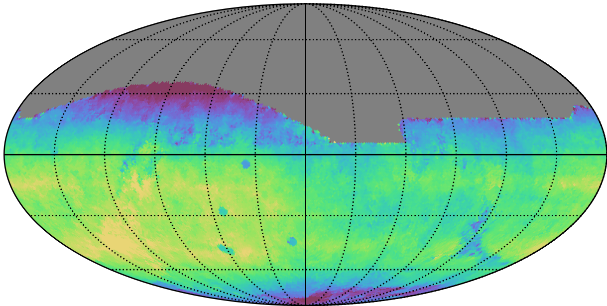
too_5_1v3.4_10yrs All sky r band: Median fiveSigmaDepth
