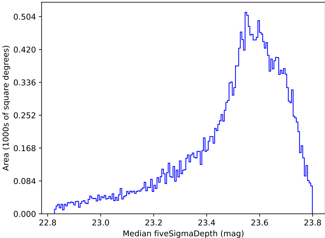
too_5_1v3.4_10yrs All sky i band: Median fiveSigmaDepth
