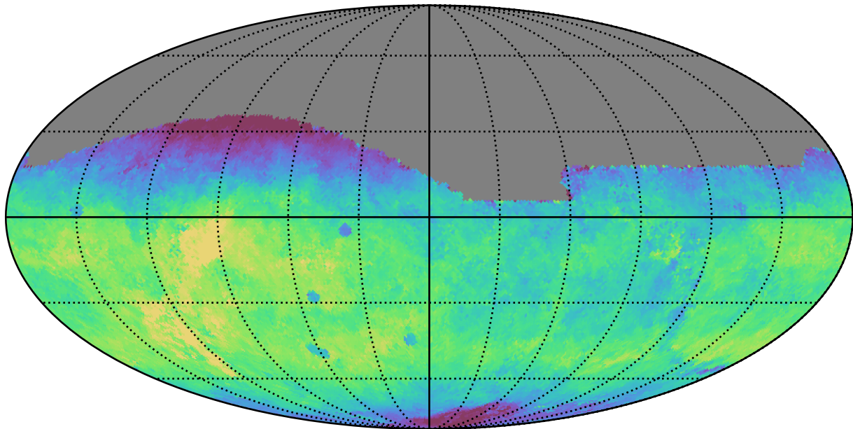
too_5_1v3.4_10yrs All sky g band: Median fiveSigmaDepth
