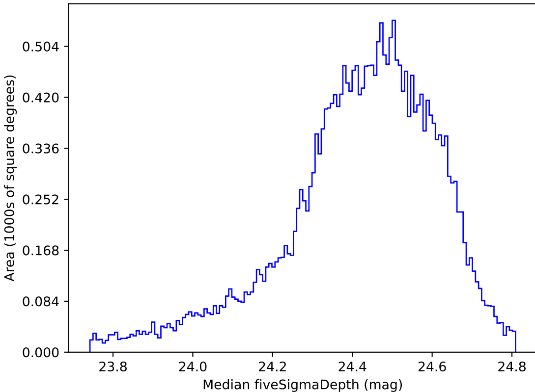
too_5_1v3.4_10yrs All sky g band: Median fiveSigmaDepth
