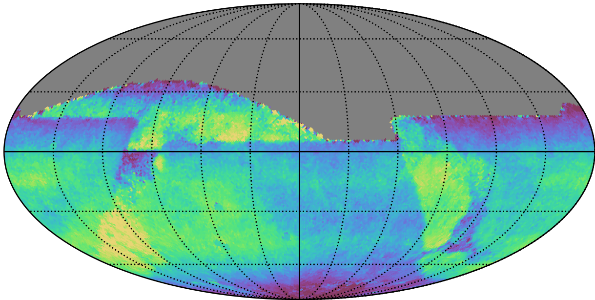
too_5_1v3.4_10yrs All sky all bands: Median fiveSigmaDepth
