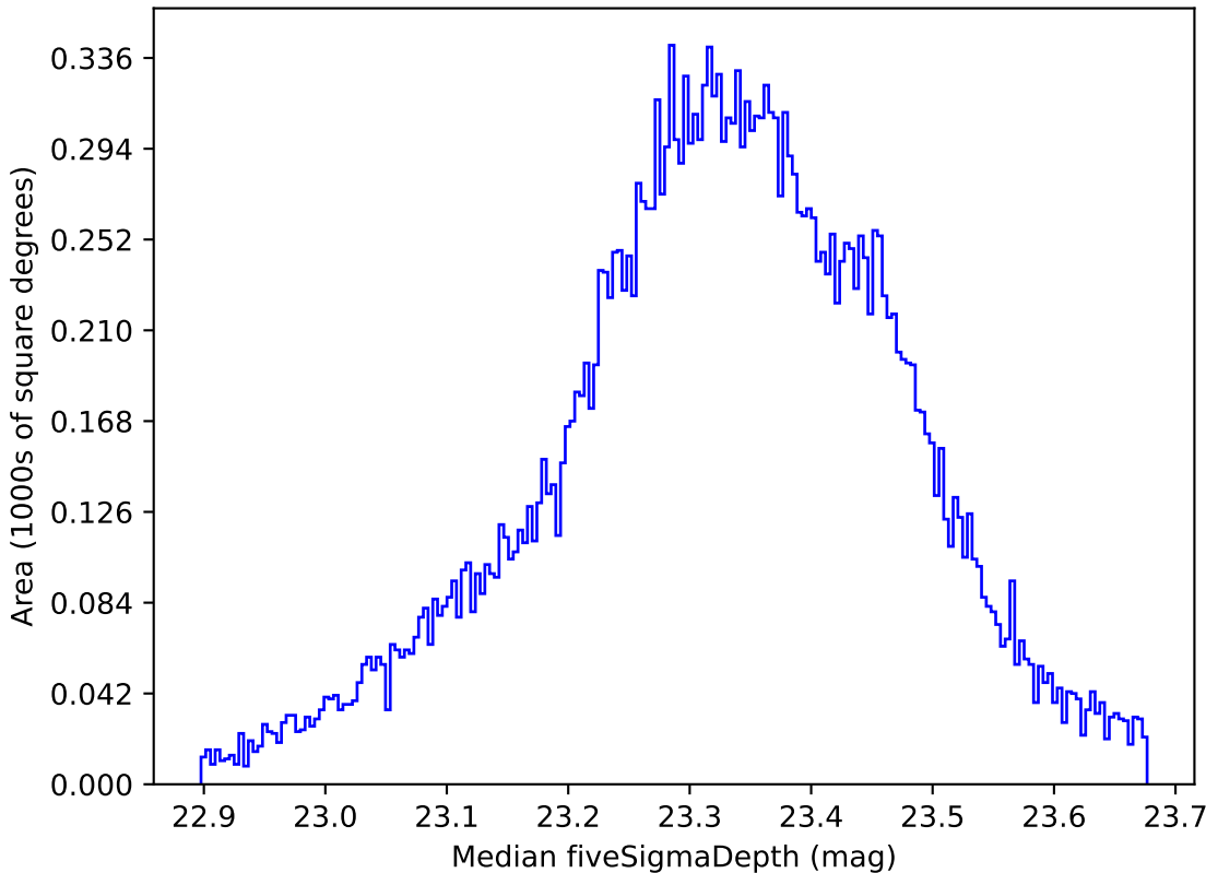
too_5_1v3.4_10yrs All sky all bands: Median fiveSigmaDepth
