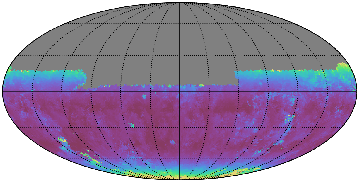
too_5_1v3.4_10yrs Yr 1 y band: Median airmass
