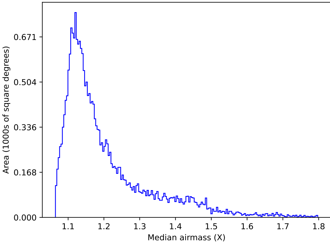
too_5_1v3.4_10yrs Yr 1 y band: Median airmass
