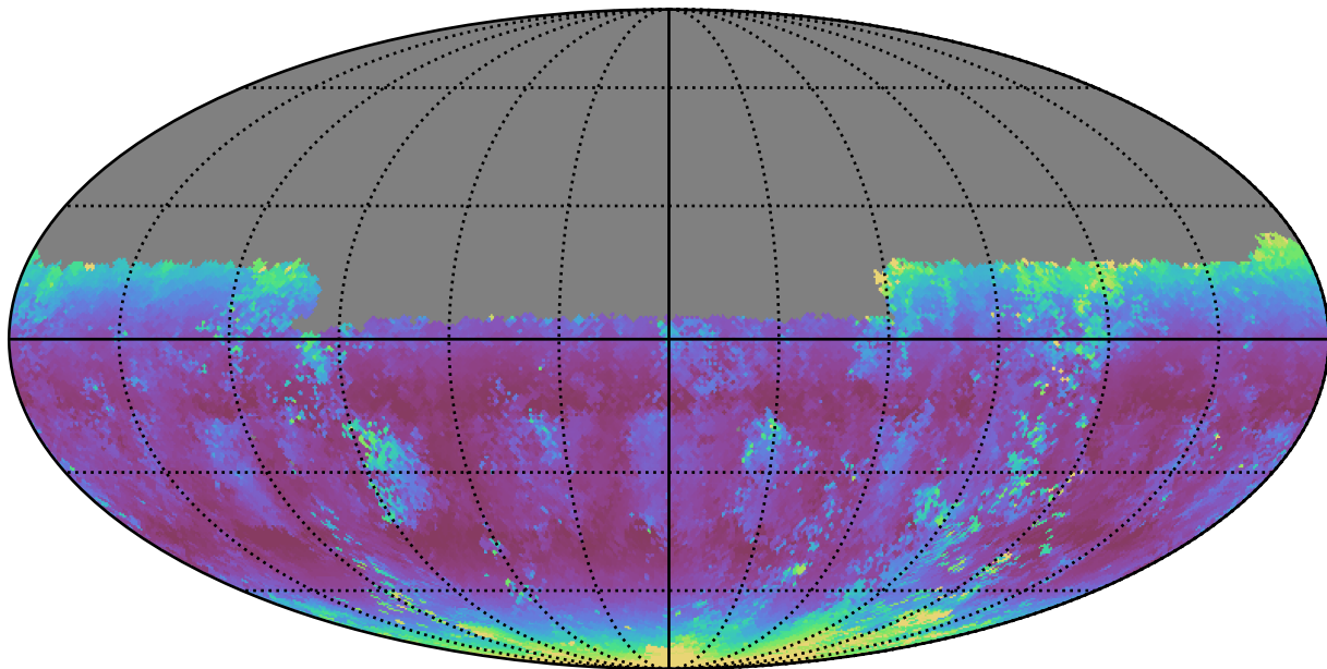
too_5_1v3.4_10yrs Yr 1 u band: Median airmass
