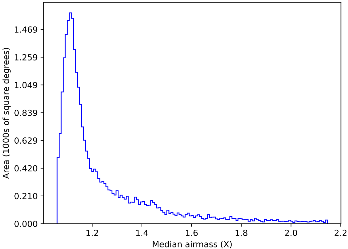
too_5_1v3.4_10yrs Yr 1 r band: Median airmass
