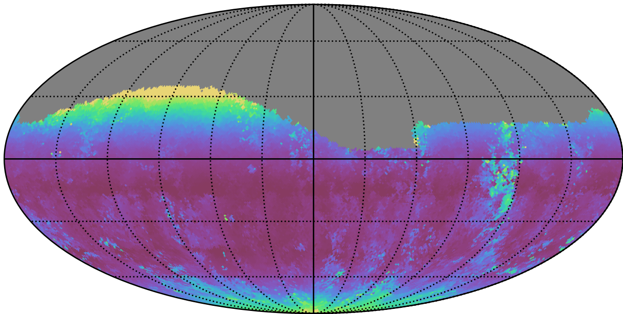
too_5_1v3.4_10yrs Yr 1 g band: Median airmass
