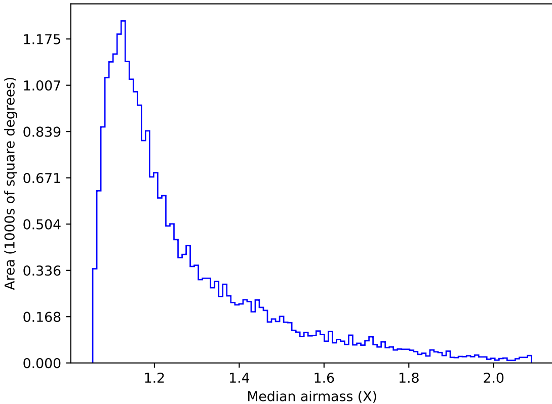
too_5_1v3.4_10yrs Yr 1 g band: Median airmass
