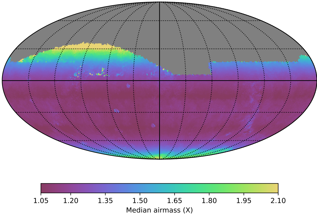
too_5_1v3.4_10yrs Yr 1 all bands: Median airmass
