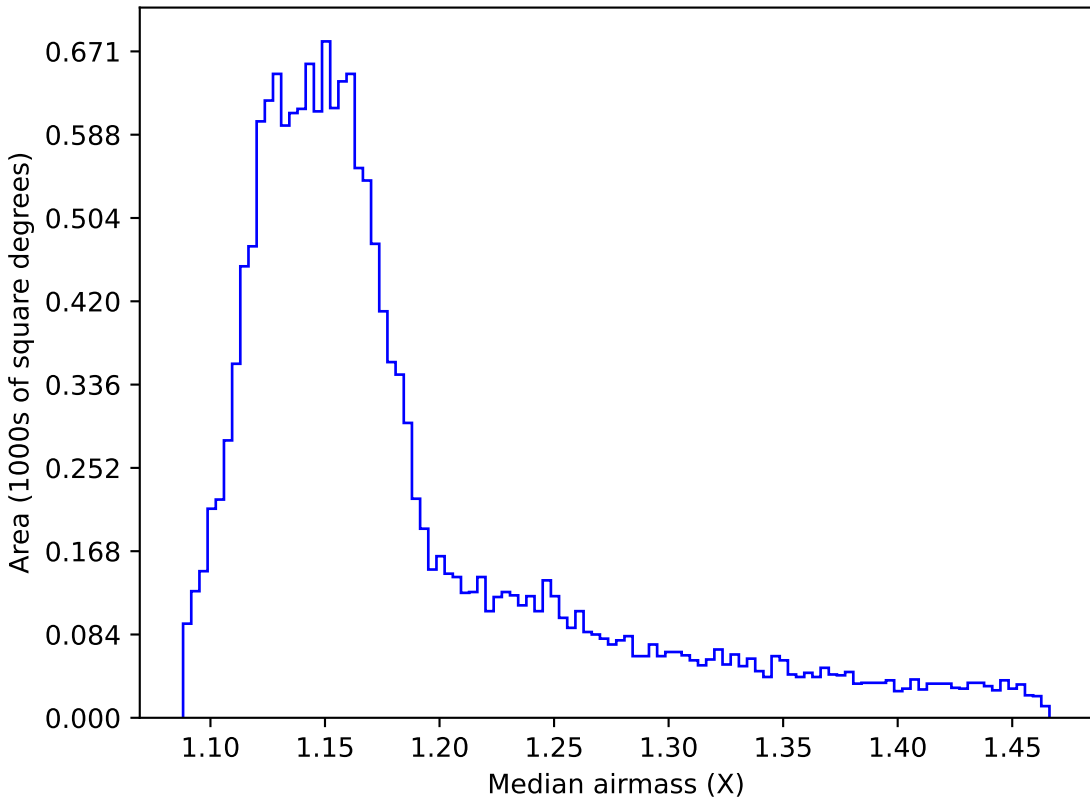
too_5_1v3.4_10yrs WFD z band: Median airmass
