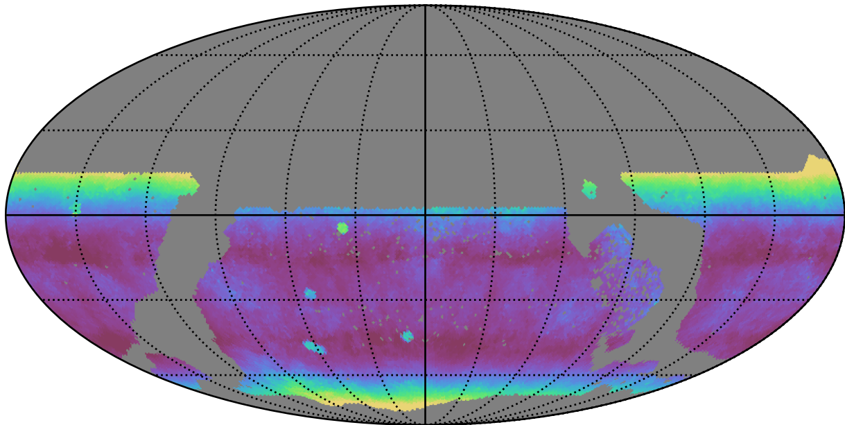
too_5_1v3.4_10yrs WFD y band: Median airmass
