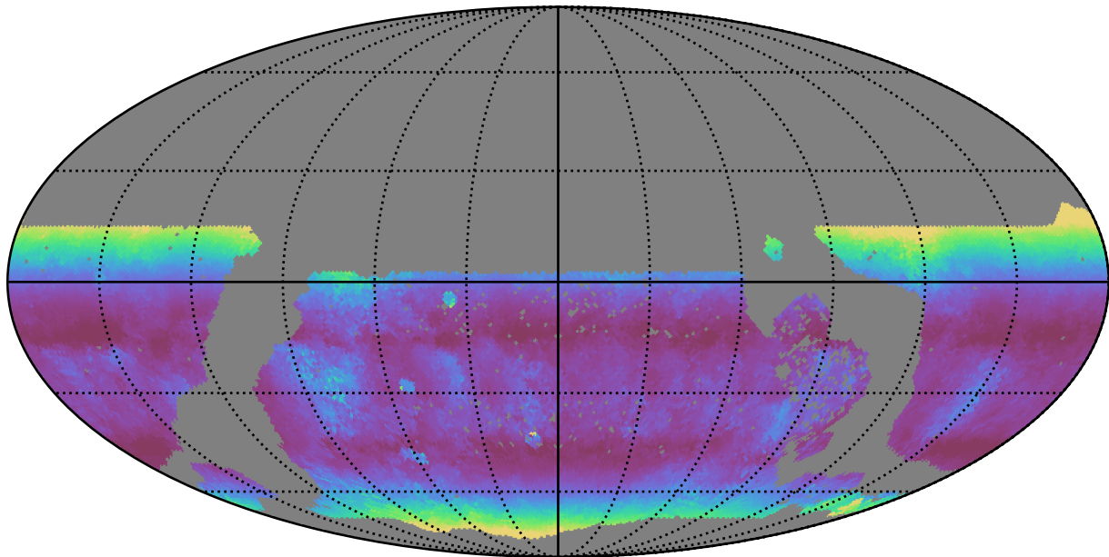
too_5_1v3.4_10yrs WFD u band: Median airmass
