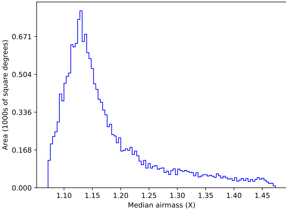
too_5_1v3.4_10yrs WFD u band: Median airmass
