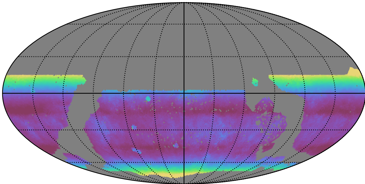
too_5_1v3.4_10yrs WFD i band: Median airmass
