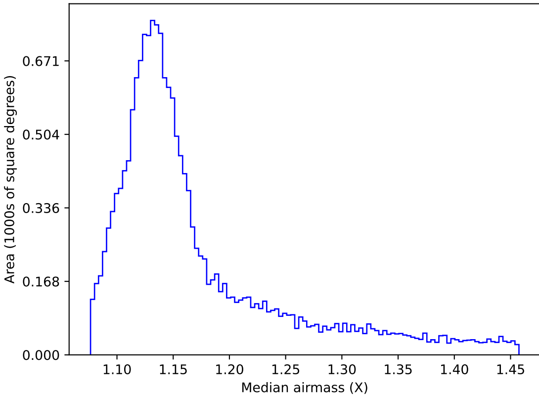
too_5_1v3.4_10yrs WFD i band: Median airmass
