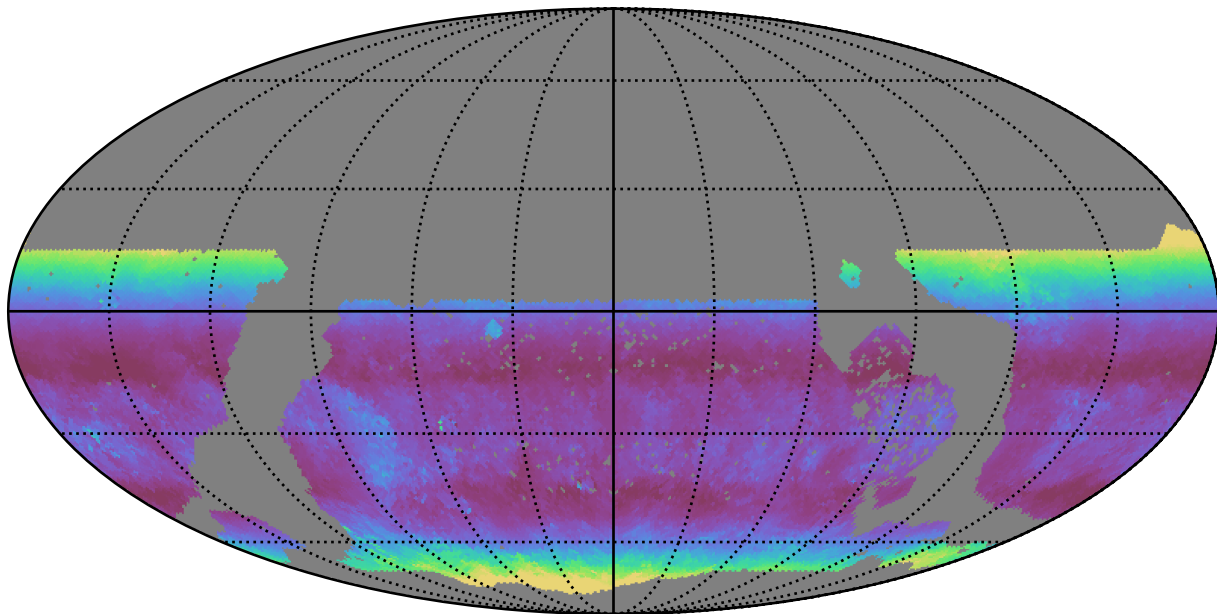
too_5_1v3.4_10yrs WFD g band: Median airmass
