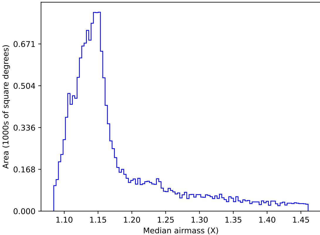
too_5_1v3.4_10yrs WFD all bands: Median airmass
