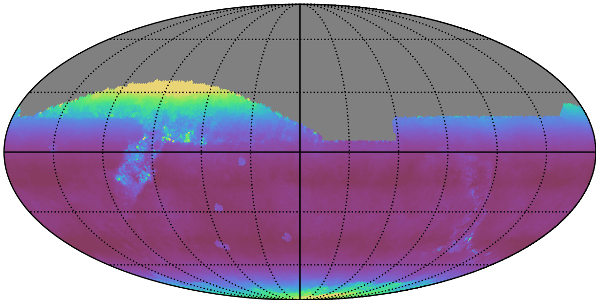
too_5_1v3.4_10yrs All sky z band: Median airmass
