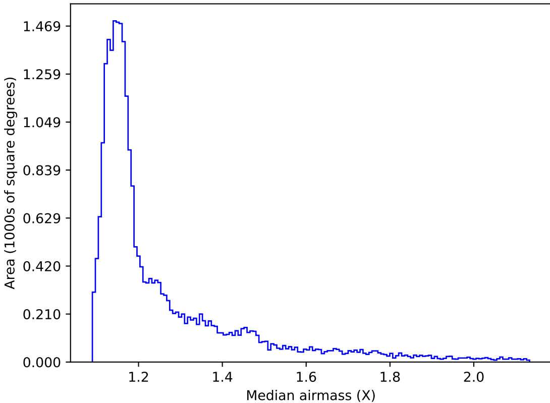
too_5_1v3.4_10yrs All sky z band: Median airmass
