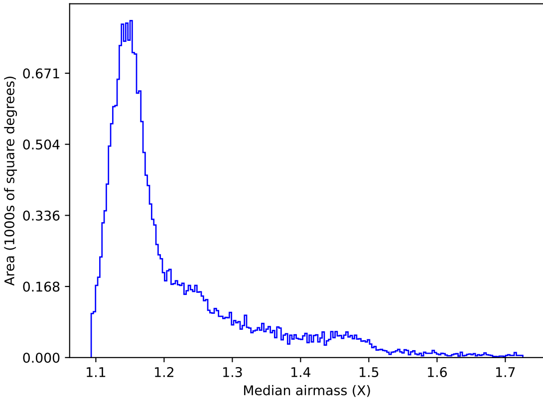
too_5_1v3.4_10yrs All sky y band: Median airmass
