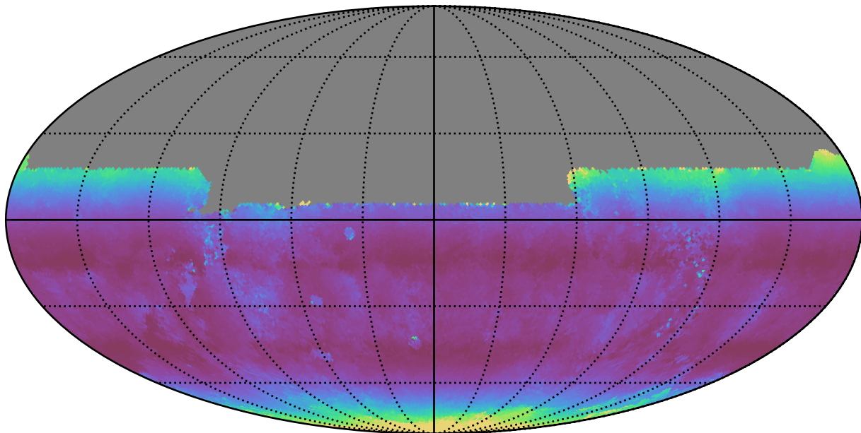
too_5_1v3.4_10yrs All sky u band: Median airmass
