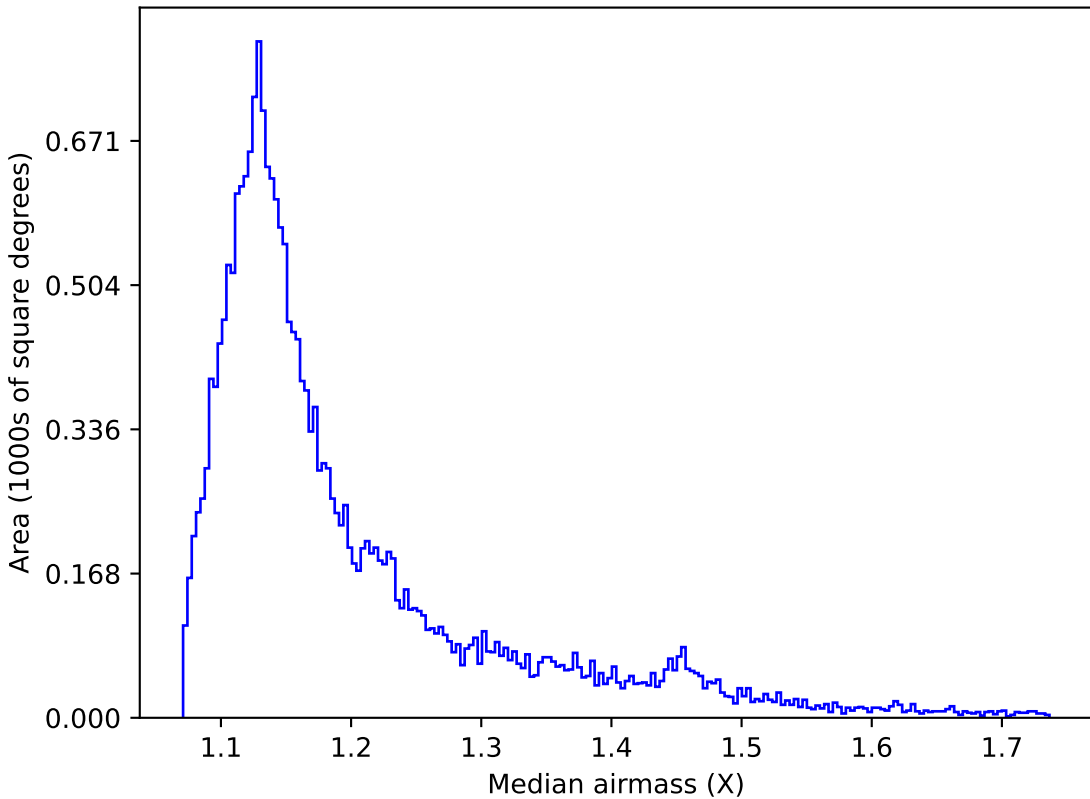
too_5_1v3.4_10yrs All sky u band: Median airmass
